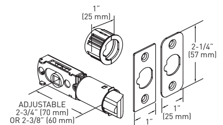
6-IN-1 ENTRY LATCH
