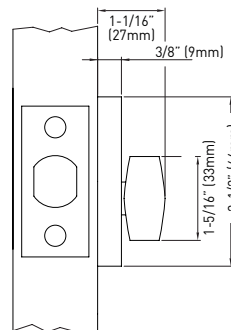
SINGLE SIDED INTERIOR DEADBOLT
