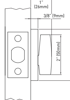
INSIDE TRIM DEADBOLT
