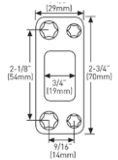
HIGH SECURITY STRIKE
